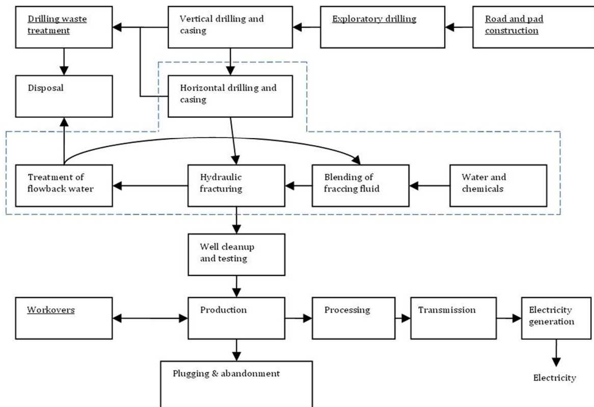
Figure 3.2: Detailed process diagram of the shale gas electricity generation system. Main differences with the conventional gas system described in section 3.1 are indicated in the blue dashed box. Processes that occur in both systems, but with different requirements and/or outputs are indicated with underlined text.
