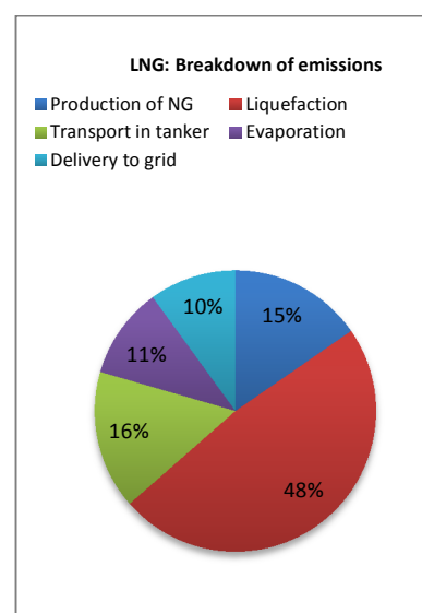
Figure 4.4: Breakdown of the GHG emissions of LNG production, transport, and delivery to the Dutch gas grid.
